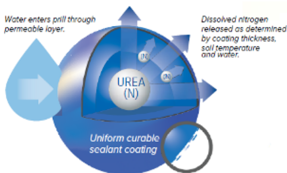
Nitrogen release mechanism in AccuBlu technology
